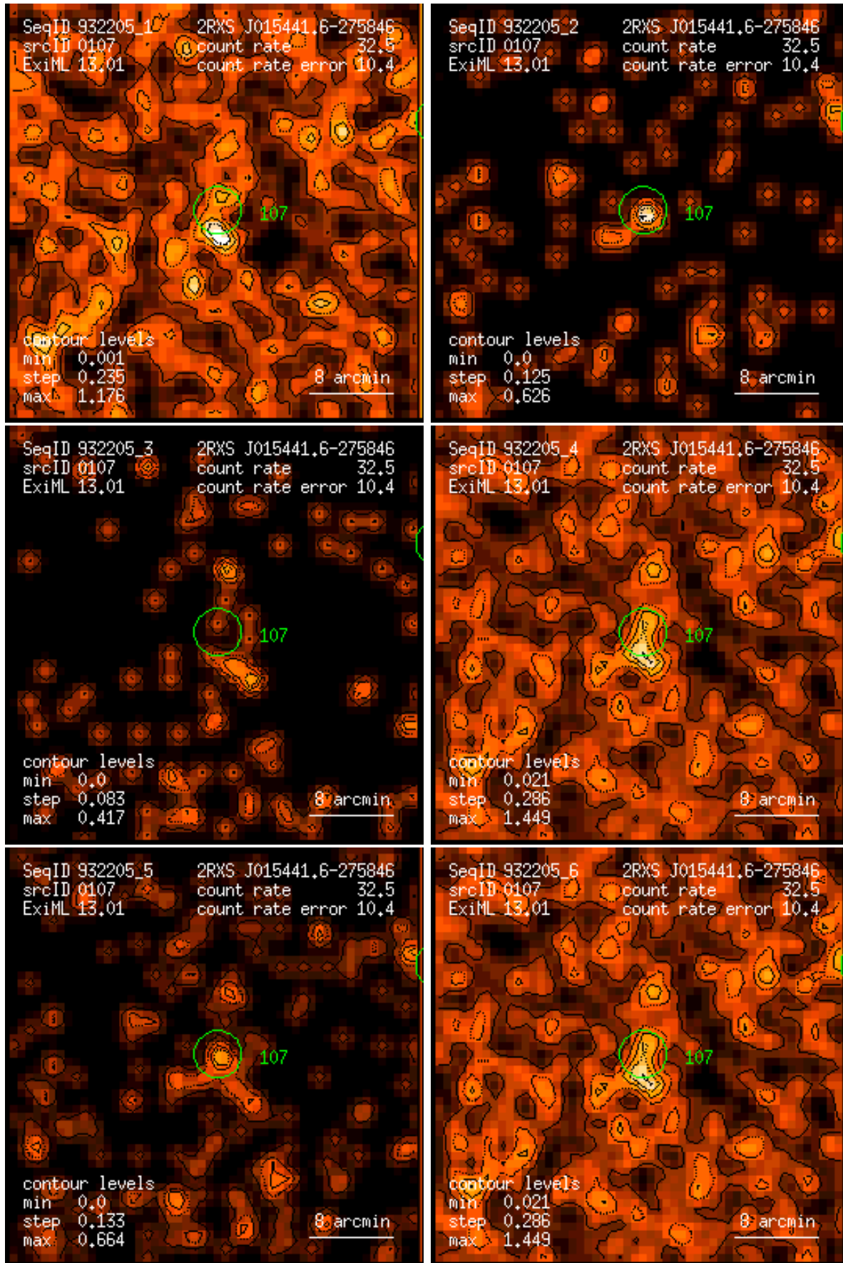
Figure 107: RASS 932205: detection 0107: band rate images, Gaussian filter: (1) PSPC channels 11 – 41, (2) 52 – 90, (3) 91 – 201, (4) 11 – 235, (5) 52 – 201, (6) 11 – 201. Broad band rates in counts/ks. Band rate contour levels in counts/ks/arcmin 2 .
