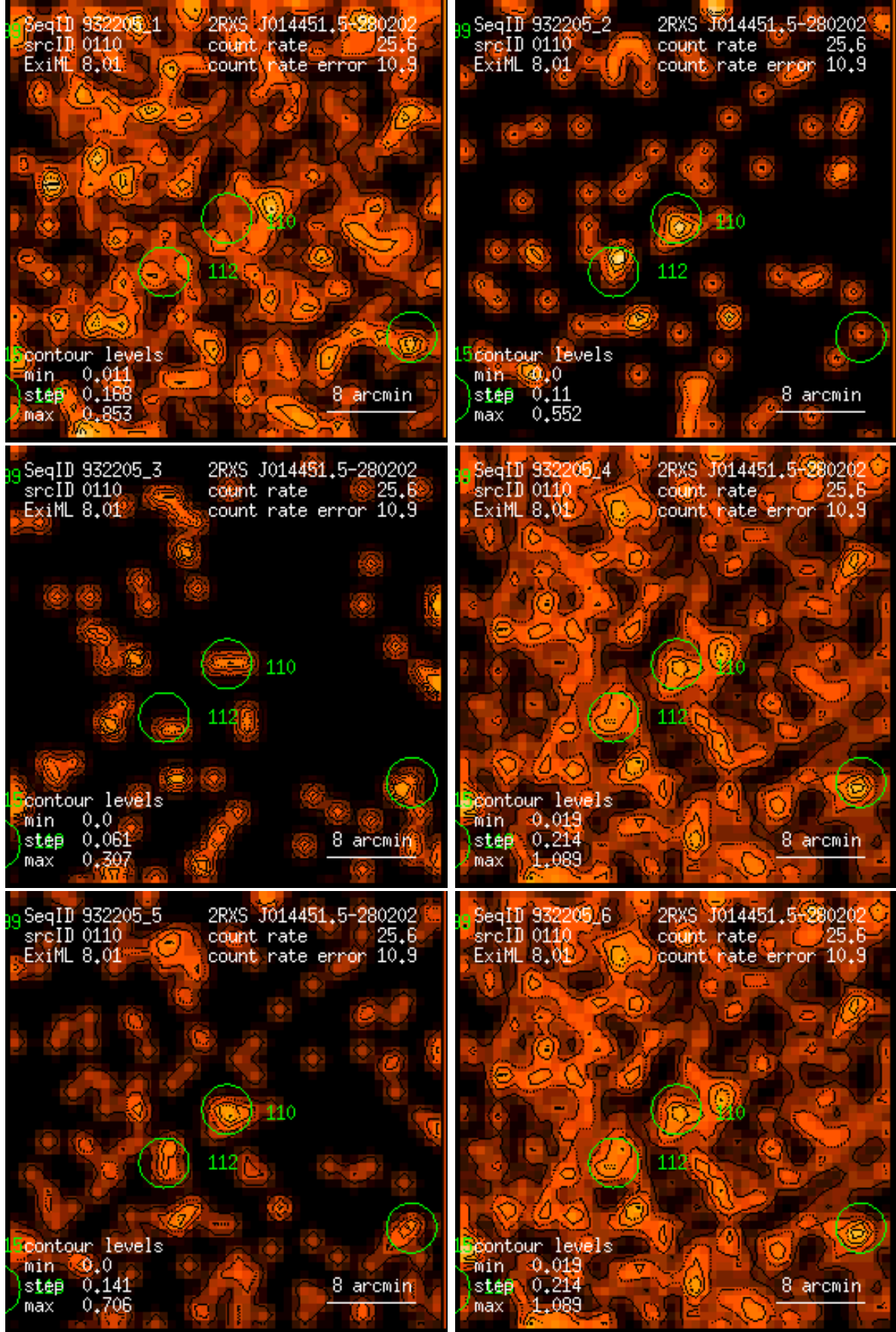
Figure 110: RASS 932205: detection 0110: band rate images, Gaussian filter: (1) PSPC channels 11 – 41, (2) 52 – 90, (3) 91 – 201, (4) 11 – 235, (5) 52 – 201, (6) 11 – 201. Broad band rates in counts/ks. Band rate contour levels in counts/ks/arcmin 2 .
