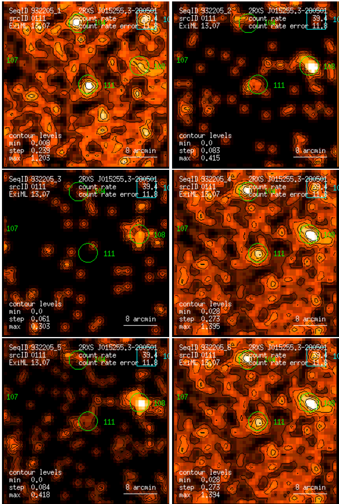
Figure 111: RASS 932205: detection 0111: band rate images, Gaussian filter: (1) PSPC channels 11 – 41, (2) 52 – 90, (3) 91 – 201, (4) 11 – 235, (5) 52 – 201, (6) 11 – 201. Broad band rates in counts/ks. Band rate contour levels in counts/ks/arcmin 2 .
