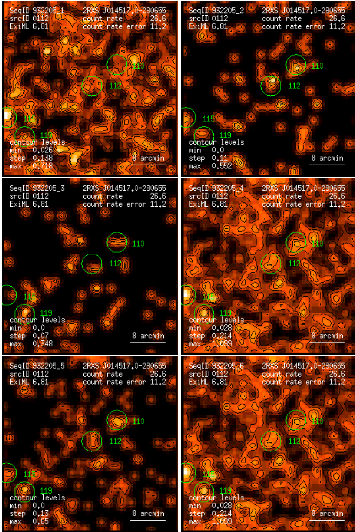
Figure 112: RASS 932205: detection 0112: band rate images, Gaussian filter: (1) PSPC channels 11 – 41, (2) 52 – 90, (3) 91 – 201, (4) 11 – 235, (5) 52 – 201, (6) 11 – 201. Broad band rates in counts/ks. Band rate contour levels in counts/ks/arcmin 2 .
