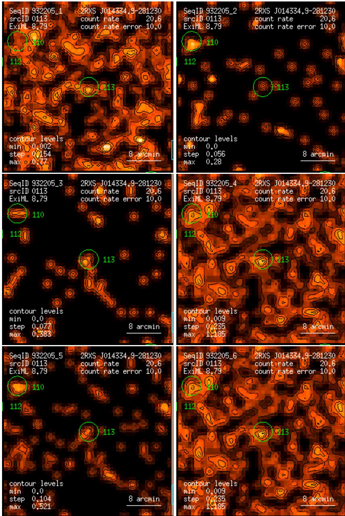
Figure 113: RASS 932205: detection 0113: band rate images, Gaussian filter: (1) PSPC channels 11 – 41, (2) 52 – 90, (3) 91 – 201, (4) 11 – 235, (5) 52 – 201, (6) 11 – 201. Broad band rates in counts/ks. Band rate contour levels in counts/ks/arcmin 2 .
