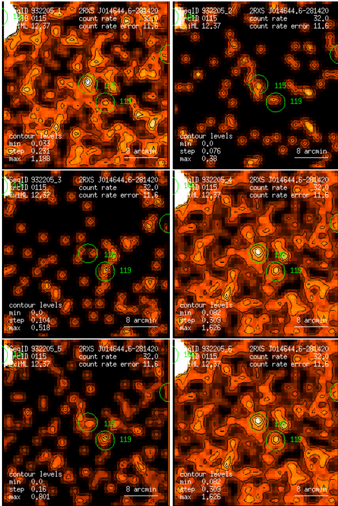
Figure 115: RASS 932205: detection 0115: band rate images, Gaussian filter: (1) PSPC channels 11 – 41, (2) 52 – 90, (3) 91 – 201, (4) 11 – 235, (5) 52 – 201, (6) 11 – 201. Broad band rates in counts/ks. Band rate contour levels in counts/ks/arcmin 2 .
