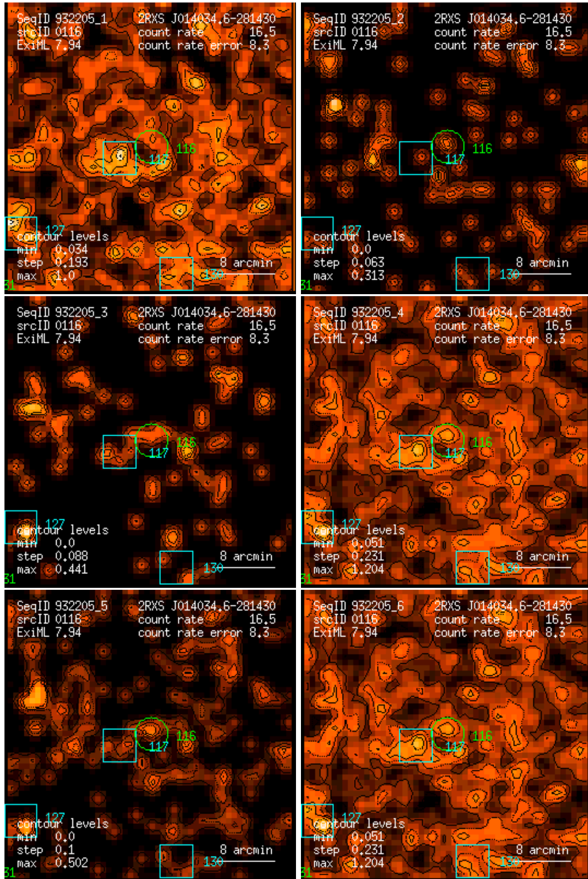
Figure 116: RASS 932205: detection 0116: band rate images, Gaussian filter: (1) PSPC channels 11 – 41, (2) 52 – 90, (3) 91 – 201, (4) 11 – 235, (5) 52 – 201, (6) 11 – 201. Broad band rates in counts/ks. Band rate contour levels in counts/ks/arcmin 2 .
