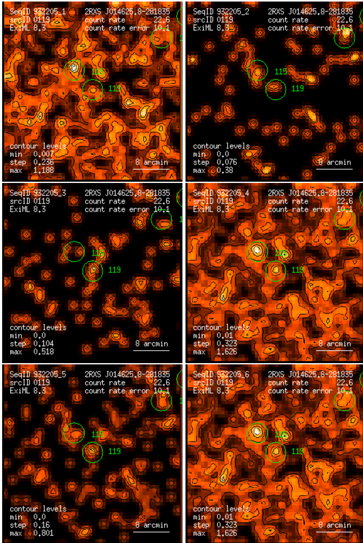
Figure 119: RASS 932205: detection 0119: band rate images, Gaussian filter: (1) PSPC channels 11 – 41, (2) 52 – 90, (3) 91 – 201, (4) 11 – 235, (5) 52 – 201, (6) 11 – 201. Broad band rates in counts/ks. Band rate contour levels in counts/ks/arcmin 2 .
