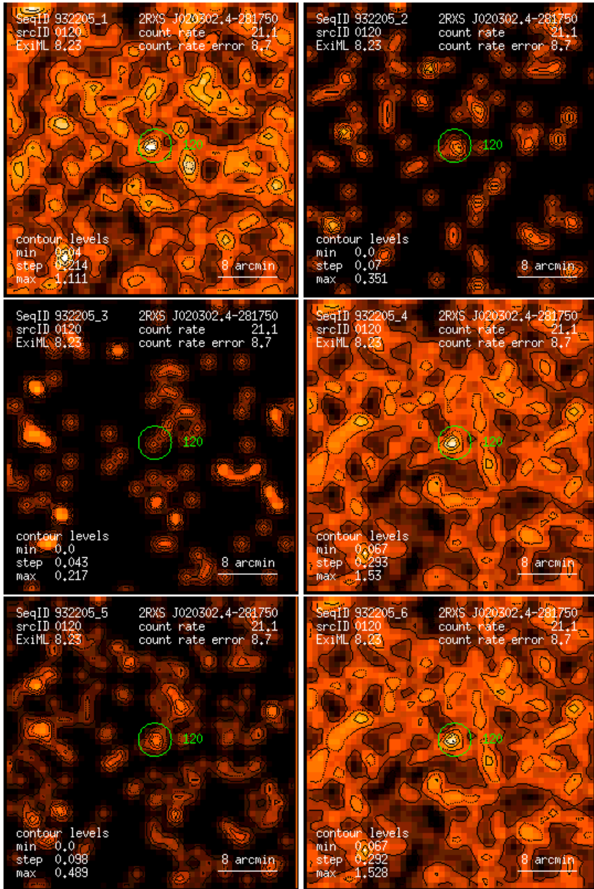
Figure 120: RASS 932205: detection 0120: band rate images, Gaussian filter: (1) PSPC channels 11 – 41, (2) 52 – 90, (3) 91 – 201, (4) 11 – 235, (5) 52 – 201, (6) 11 – 201. Broad band rates in counts/ks. Band rate contour levels in counts/ks/arcmin 2 .
