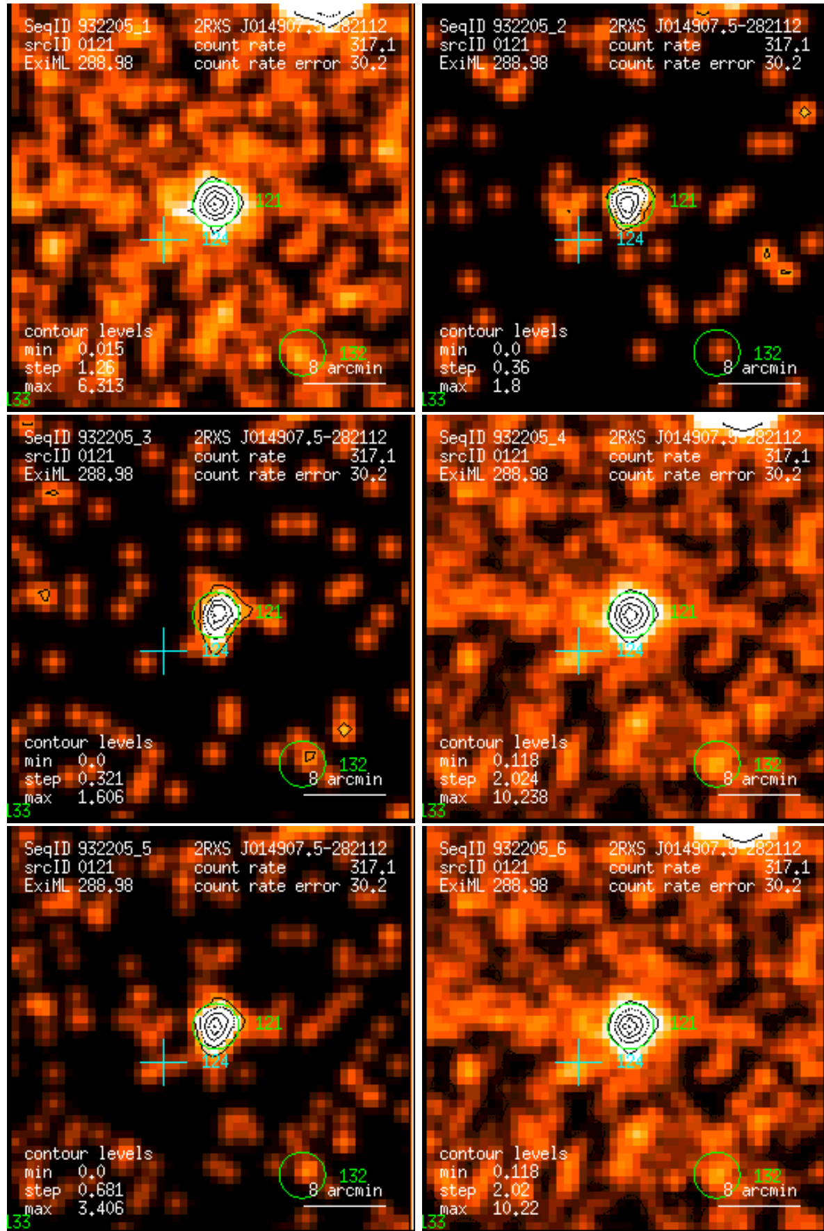
Figure 121: RASS 932205: detection 0121: band rate images, Gaussian filter: (1) PSPC channels 11 – 41, (2) 52 – 90, (3) 91 – 201, (4) 11 – 235, (5) 52 – 201, (6) 11 – 201. Broad band rates in counts/ks. Band rate contour levels in counts/ks/arcmin 2 .
