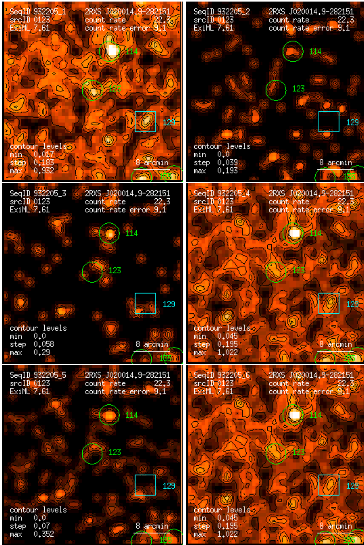
Figure 123: RASS 932205: detection 0123: band rate images, Gaussian filter: (1) PSPC channels 11 – 41, (2) 52 – 90, (3) 91 – 201, (4) 11 – 235, (5) 52 – 201, (6) 11 – 201. Broad band rates in counts/ks. Band rate contour levels in counts/ks/arcmin 2 .
