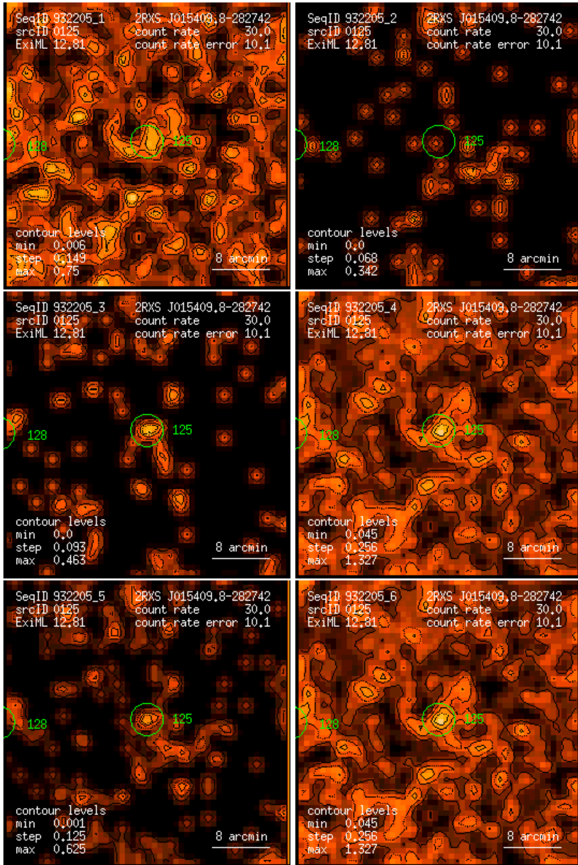
Figure 125: RASS 932205: detection 0125: band rate images, Gaussian filter: (1) PSPC channels 11 – 41, (2) 52 – 90, (3) 91 – 201, (4) 11 – 235, (5) 52 – 201, (6) 11 – 201. Broad band rates in counts/ks. Band rate contour levels in counts/ks/arcmin 2 .
