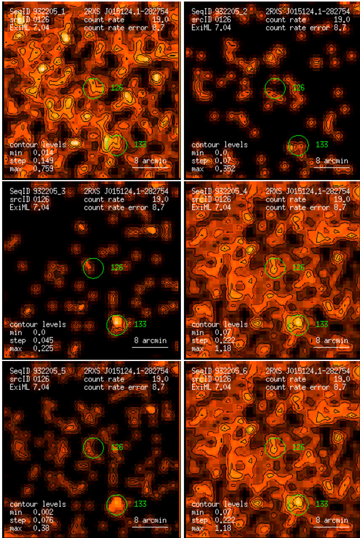
Figure 126: RASS 932205: detection 0126: band rate images, Gaussian filter: (1) PSPC channels 11 – 41, (2) 52 – 90, (3) 91 – 201, (4) 11 – 235, (5) 52 – 201, (6) 11 – 201. Broad band rates in counts/ks. Band rate contour levels in counts/ks/arcmin 2 .
