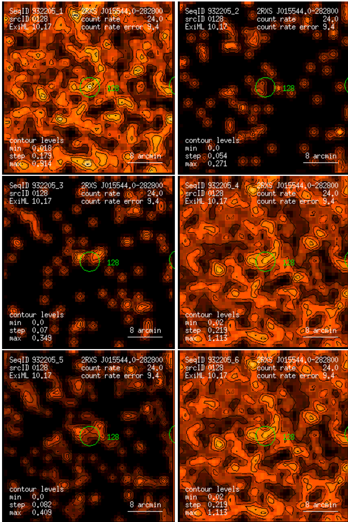
Figure 128: RASS 932205: detection 0128: band rate images, Gaussian filter: (1) PSPC channels 11 – 41, (2) 52 – 90, (3) 91 – 201, (4) 11 – 235, (5) 52 – 201, (6) 11 – 201. Broad band rates in counts/ks. Band rate contour levels in counts/ks/arcmin 2 .
