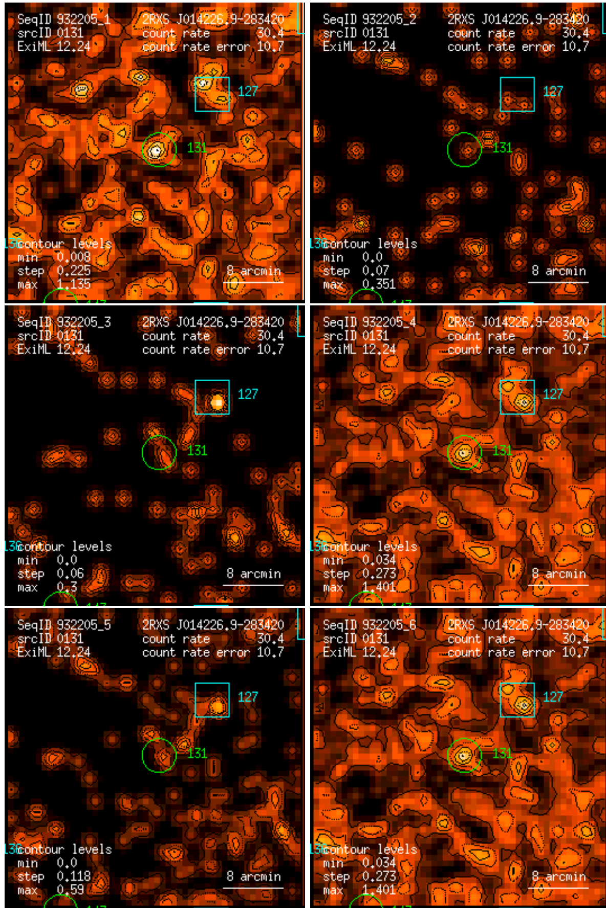
Figure 131: RASS 932205: detection 0131: band rate images, Gaussian filter: (1) PSPC channels 11 – 41, (2) 52 – 90, (3) 91 – 201, (4) 11 – 235, (5) 52 – 201, (6) 11 – 201. Broad band rates in counts/ks. Band rate contour levels in counts/ks/arcmin 2 .
