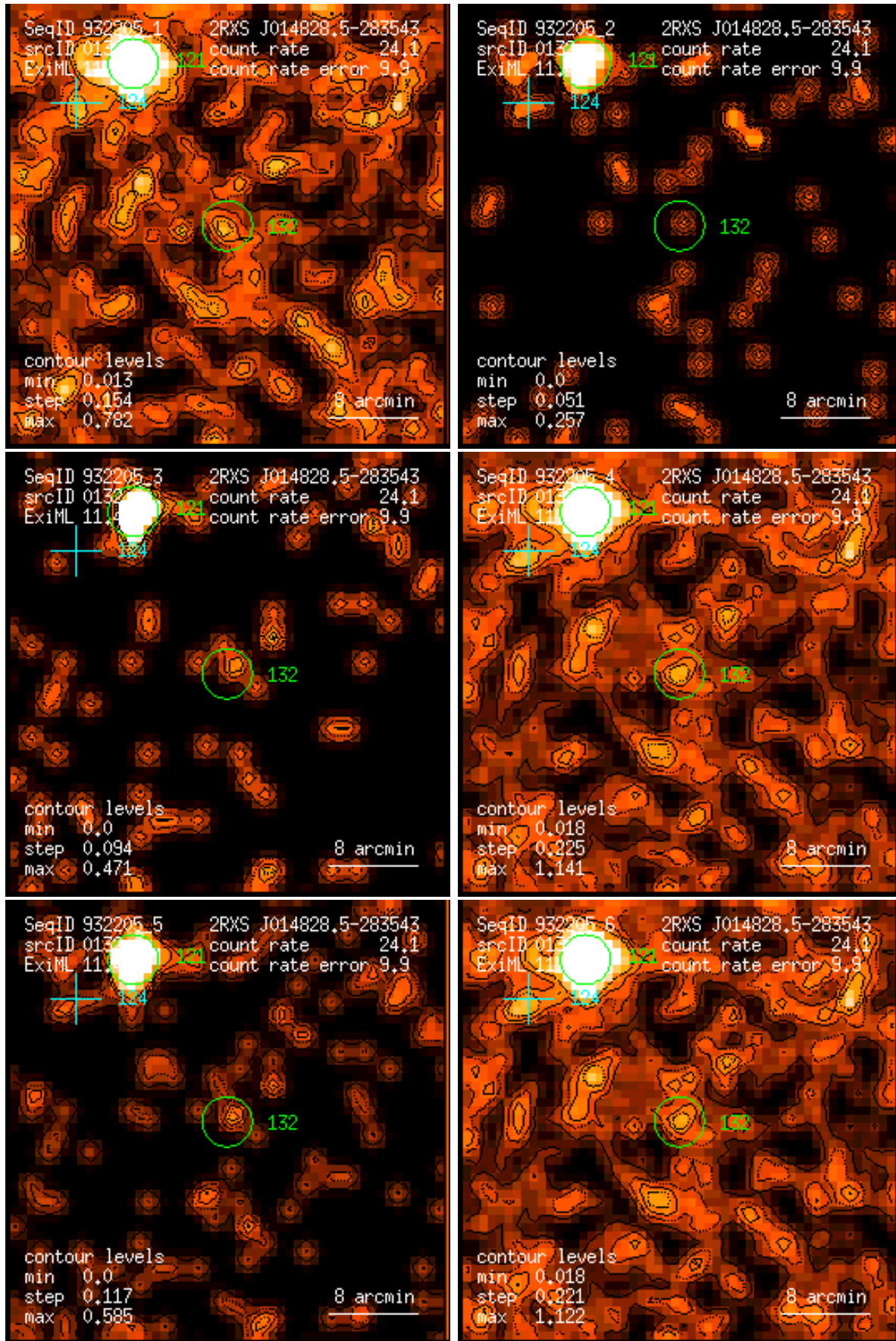
Figure 132: RASS 932205: detection 0132: band rate images, Gaussian filter: (1) PSPC channels 11 – 41, (2) 52 – 90, (3) 91 – 201, (4) 11 – 235, (5) 52 – 201, (6) 11 – 201. Broad band rates in counts/ks. Band rate contour levels in counts/ks/arcmin 2 .
