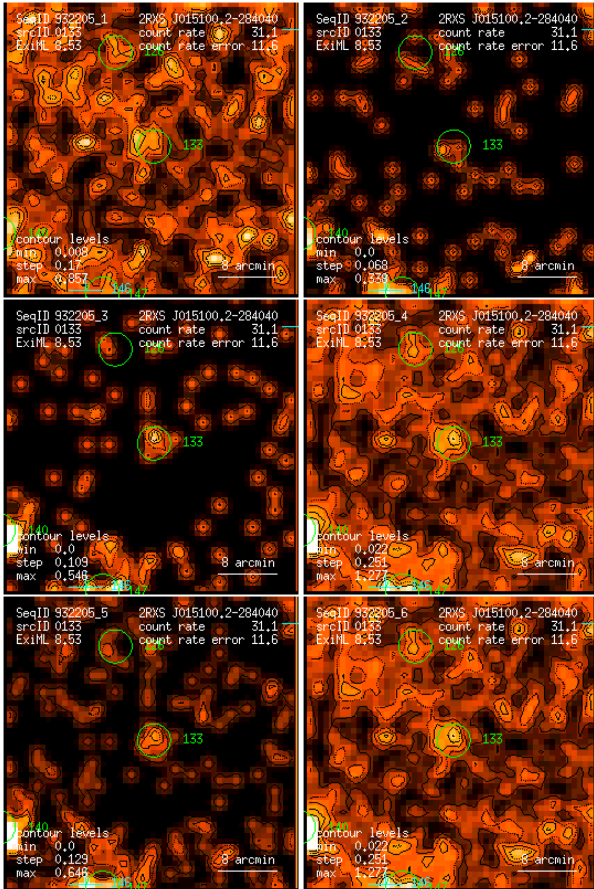
Figure 133: RASS 932205: detection 0133: band rate images, Gaussian filter: (1) PSPC channels 11 – 41, (2) 52 – 90, (3) 91 – 201, (4) 11 – 235, (5) 52 – 201, (6) 11 – 201. Broad band rates in counts/ks. Band rate contour levels in counts/ks/arcmin 2 .
