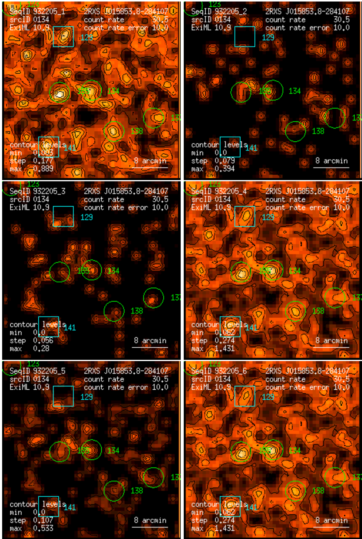
Figure 134: RASS 932205: detection 0134: band rate images, Gaussian filter: (1) PSPC channels 11 – 41, (2) 52 – 90, (3) 91 – 201, (4) 11 – 235, (5) 52 – 201, (6) 11 – 201. Broad band rates in counts/ks. Band rate contour levels in counts/ks/arcmin 2 .
