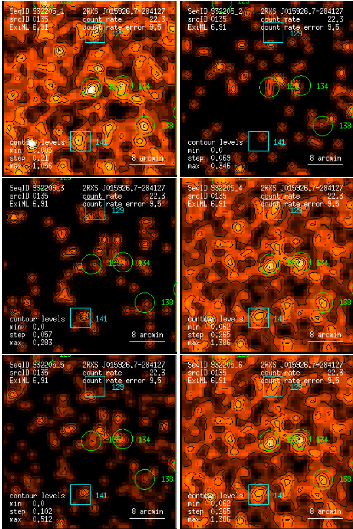
Figure 135: RASS 932205: detection 0135: band rate images, Gaussian filter: (1) PSPC channels 11 – 41, (2) 52 – 90, (3) 91 – 201, (4) 11 – 235, (5) 52 – 201, (6) 11 – 201. Broad band rates in counts/ks. Band rate contour levels in counts/ks/arcmin 2 .
