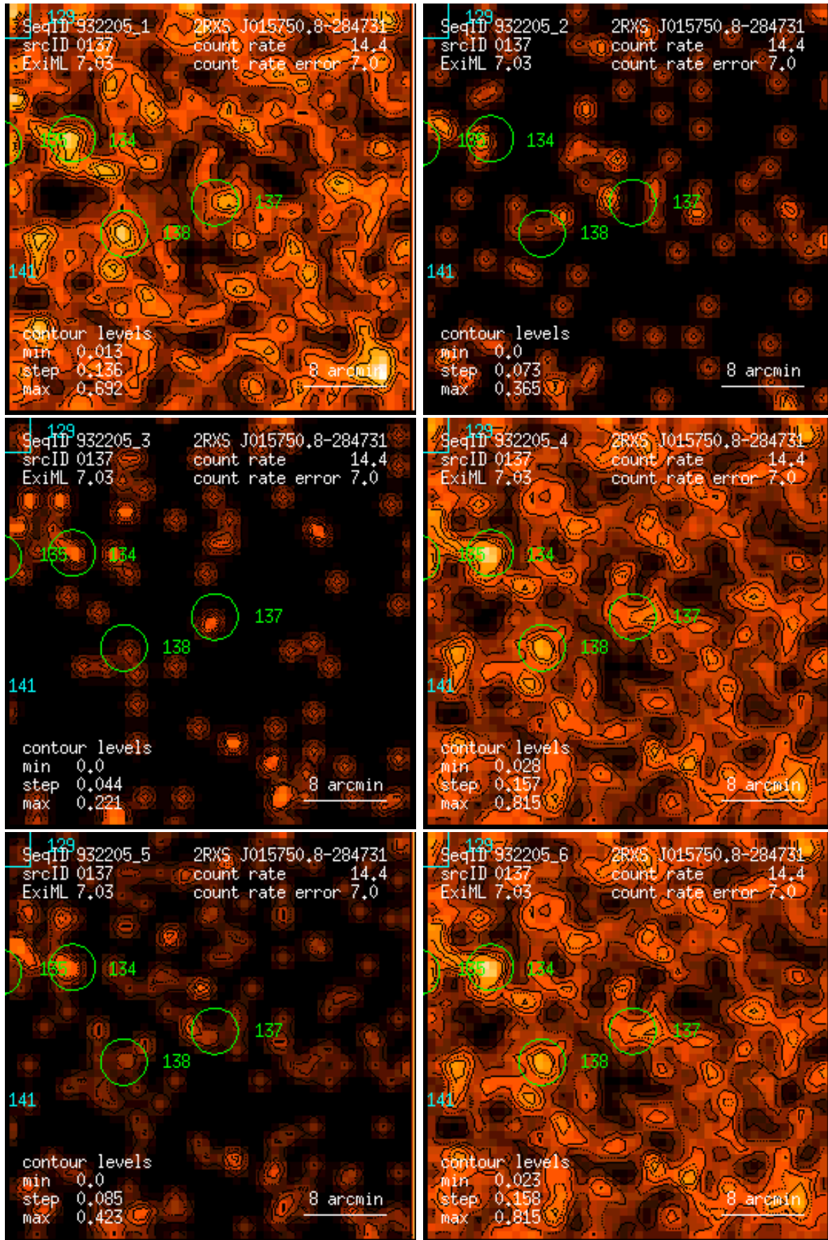
Figure 137: RASS 932205: detection 0137: band rate images, Gaussian filter: (1) PSPC channels 11 – 41, (2) 52 – 90, (3) 91 – 201, (4) 11 – 235, (5) 52 – 201, (6) 11 – 201. Broad band rates in counts/ks. Band rate contour levels in counts/ks/arcmin 2 .
