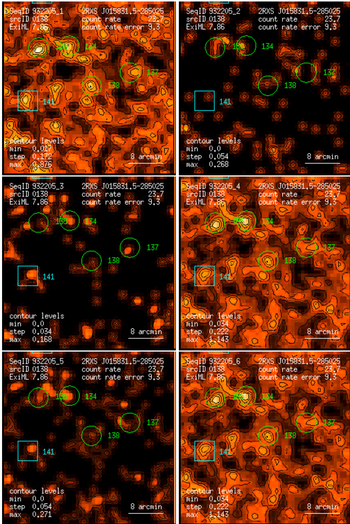
Figure 138: RASS 932205: detection 0138: band rate images, Gaussian filter: (1) PSPC channels 11 – 41, (2) 52 – 90, (3) 91 – 201, (4) 11 – 235, (5) 52 – 201, (6) 11 – 201. Broad band rates in counts/ks. Band rate contour levels in counts/ks/arcmin 2 .
