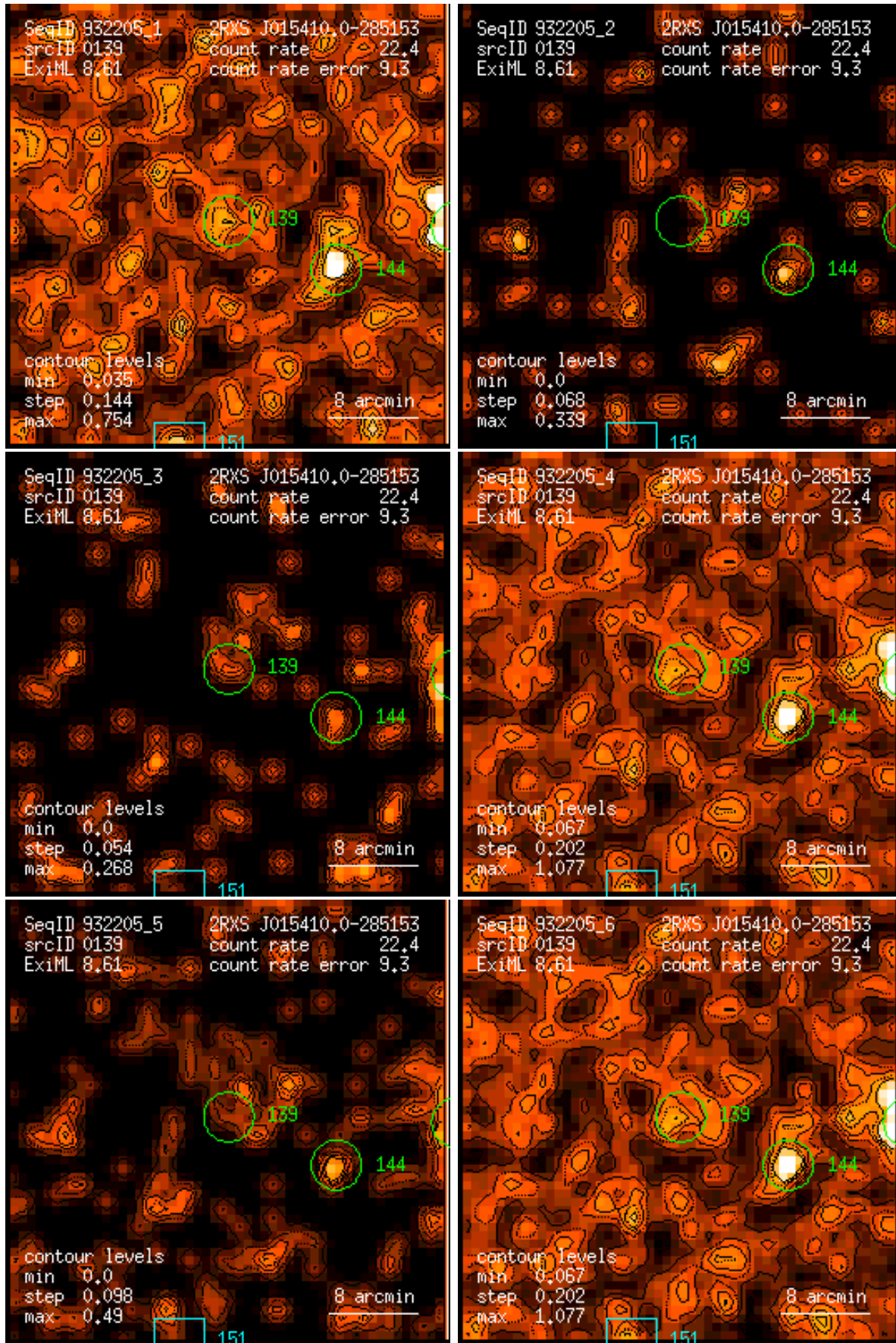
Figure 139: RASS 932205: detection 0139: band rate images, Gaussian filter: (1) PSPC channels 11 – 41, (2) 52 – 90, (3) 91 – 201, (4) 11 – 235, (5) 52 – 201, (6) 11 – 201. Broad band rates in counts/ks. Band rate contour levels in counts/ks/arcmin 2 .
