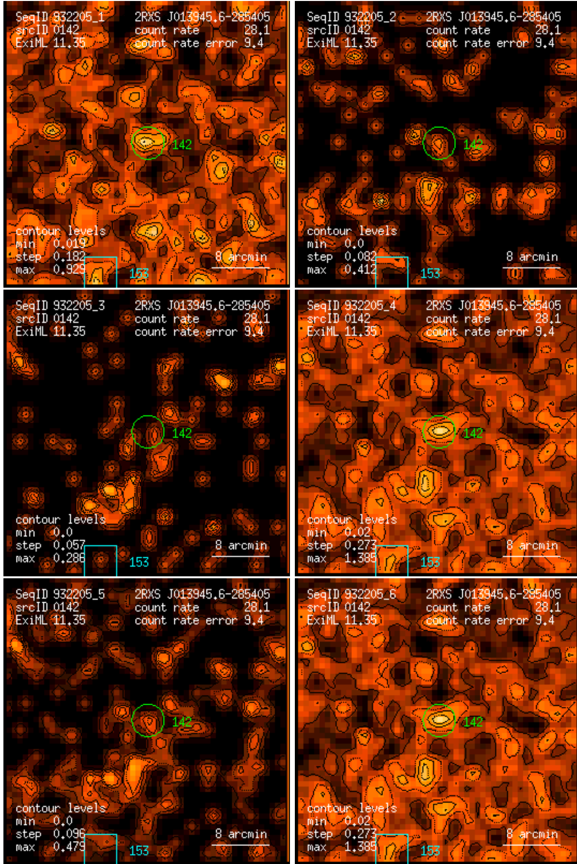
Figure 142: RASS 932205: detection 0142: band rate images, Gaussian filter: (1) PSPC channels 11 – 41, (2) 52 – 90, (3) 91 – 201, (4) 11 – 235, (5) 52 – 201, (6) 11 – 201. Broad band rates in counts/ks. Band rate contour levels in counts/ks/arcmin 2 .
