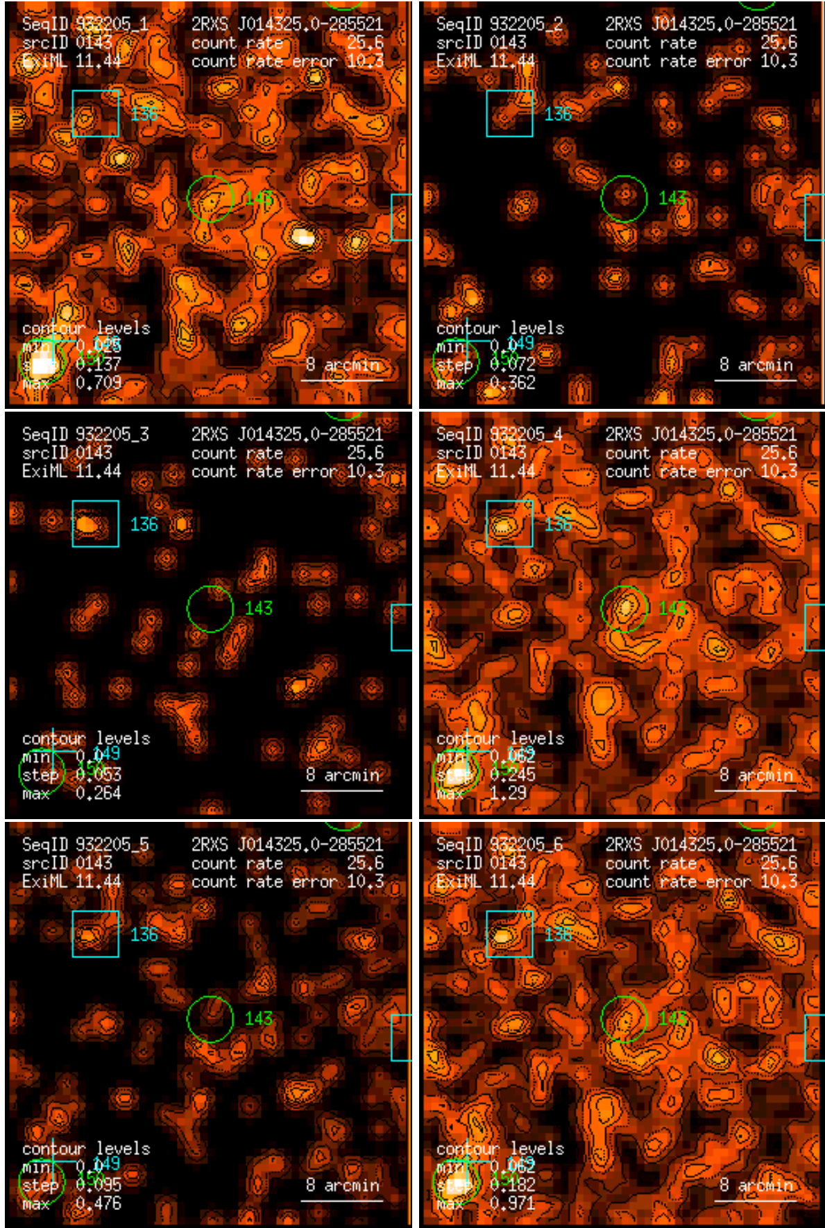
Figure 143: RASS 932205: detection 0143: band rate images, Gaussian filter: (1) PSPC channels 11 – 41, (2) 52 – 90, (3) 91 – 201, (4) 11 – 235, (5) 52 – 201, (6) 11 – 201. Broad band rates in counts/ks. Band rate contour levels in counts/ks/arcmin 2 .
