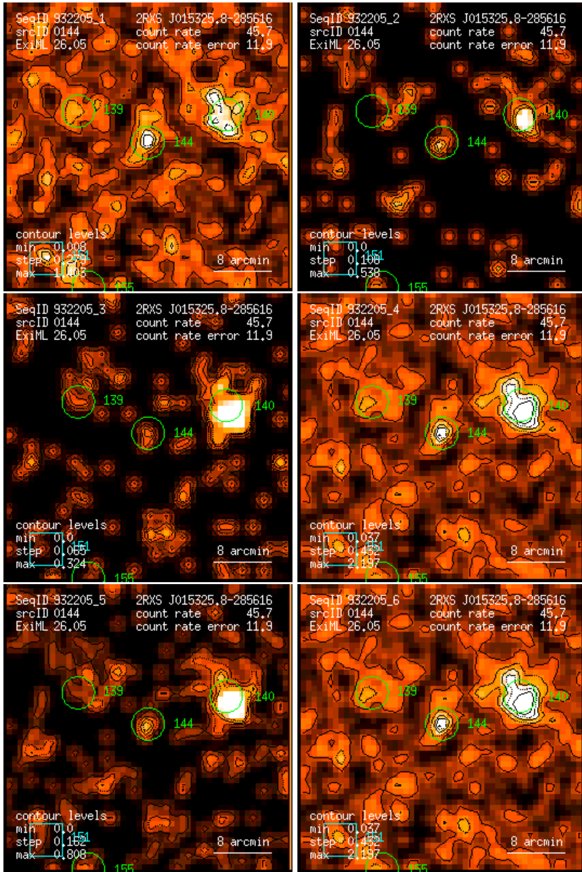
Figure 144: RASS 932205: detection 0144: band rate images, Gaussian filter: (1) PSPC channels 11 – 41, (2) 52 – 90, (3) 91 – 201, (4) 11 – 235, (5) 52 – 201, (6) 11 – 201. Broad band rates in counts/ks. Band rate contour levels in counts/ks/arcmin 2 .
