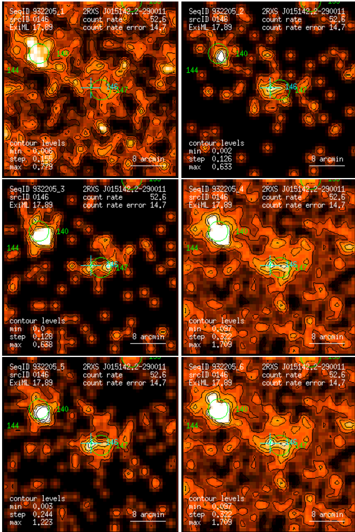
Figure 146: RASS 932205: detection 0146: band rate images, Gaussian filter: (1) PSPC channels 11 – 41, (2) 52 – 90, (3) 91 – 201, (4) 11 – 235, (5) 52 – 201, (6) 11 – 201. Broad band rates in counts/ks. Band rate contour levels in counts/ks/arcmin 2 .
