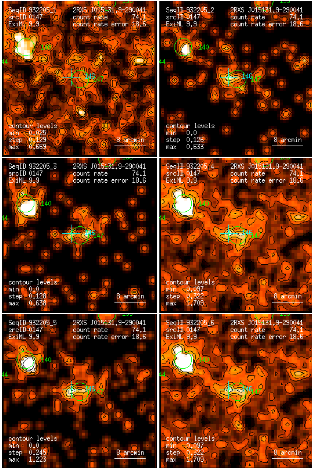
Figure 147: RASS 932205: detection 0147: band rate images, Gaussian filter: (1) PSPC channels 11 – 41, (2) 52 – 90, (3) 91 – 201, (4) 11 – 235, (5) 52 – 201, (6) 11 – 201. Broad band rates in counts/ks. Band rate contour levels in counts/ks/arcmin 2 .
