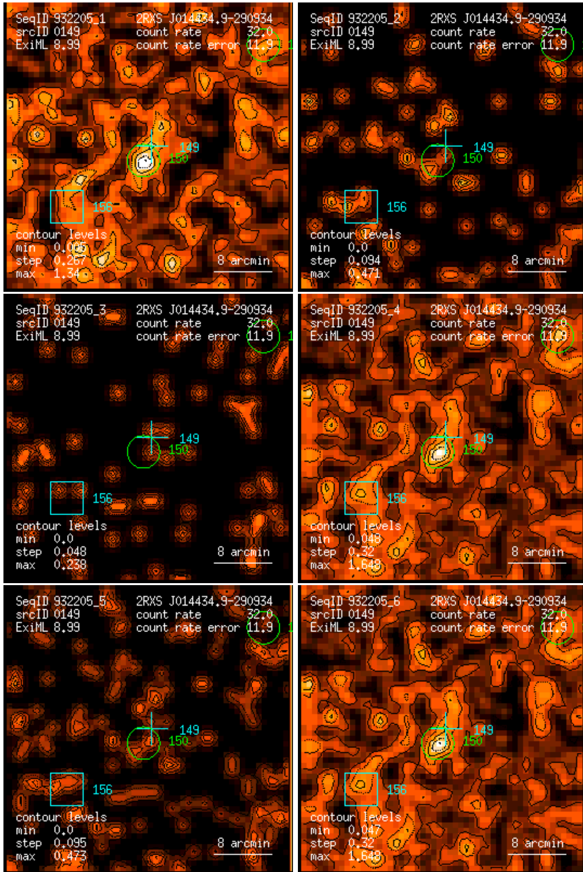
Figure 149: RASS 932205: detection 0149: band rate images, Gaussian filter: (1) PSPC channels 11 – 41, (2) 52 – 90, (3) 91 – 201, (4) 11 – 235, (5) 52 – 201, (6) 11 – 201. Broad band rates in counts/ks. Band rate contour levels in counts/ks/arcmin 2 .
