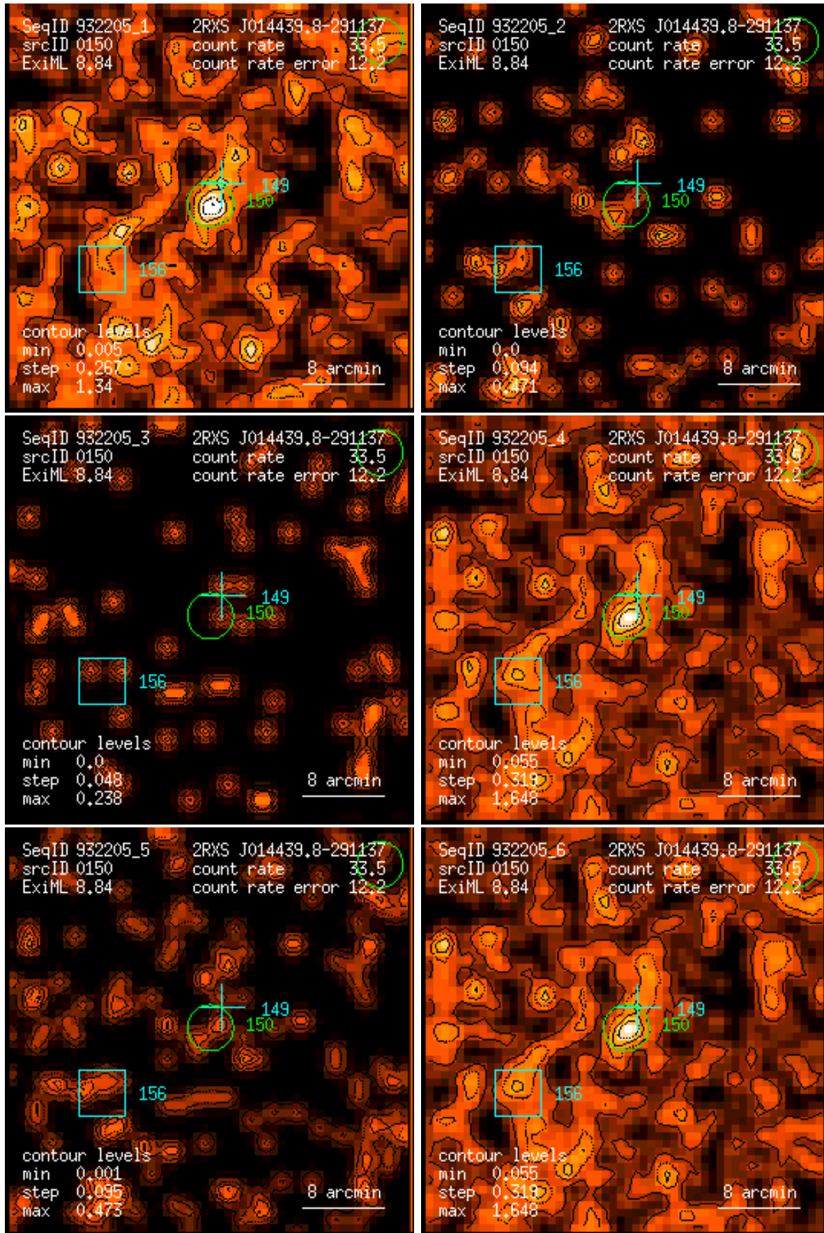
Figure 150: RASS 932205: detection 0150: band rate images, Gaussian filter: (1) PSPC channels 11 – 41, (2) 52 – 90, (3) 91 – 201, (4) 11 – 235, (5) 52 – 201, (6) 11 – 201. Broad band rates in counts/ks. Band rate contour levels in counts/ks/arcmin 2 .
