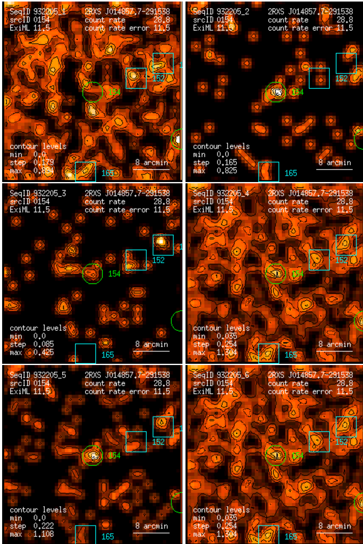
Figure 154: RASS 932205: detection 0154: band rate images, Gaussian filter: (1) PSPC channels 11 – 41, (2) 52 – 90, (3) 91 – 201, (4) 11 – 235, (5) 52 – 201, (6) 11 – 201. Broad band rates in counts/ks. Band rate contour levels in counts/ks/arcmin 2 .
