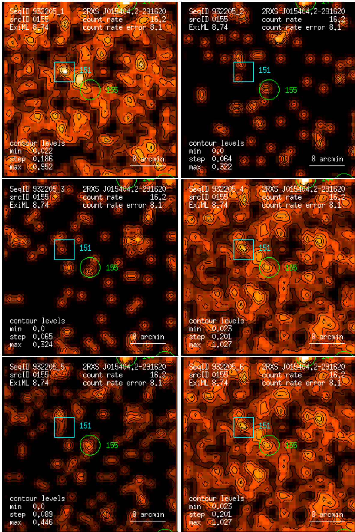
Figure 155: RASS 932205: detection 0155: band rate images, Gaussian filter: (1) PSPC channels 11 – 41, (2) 52 – 90, (3) 91 – 201, (4) 11 – 235, (5) 52 – 201, (6) 11 – 201. Broad band rates in counts/ks. Band rate contour levels in counts/ks/arcmin 2 .
