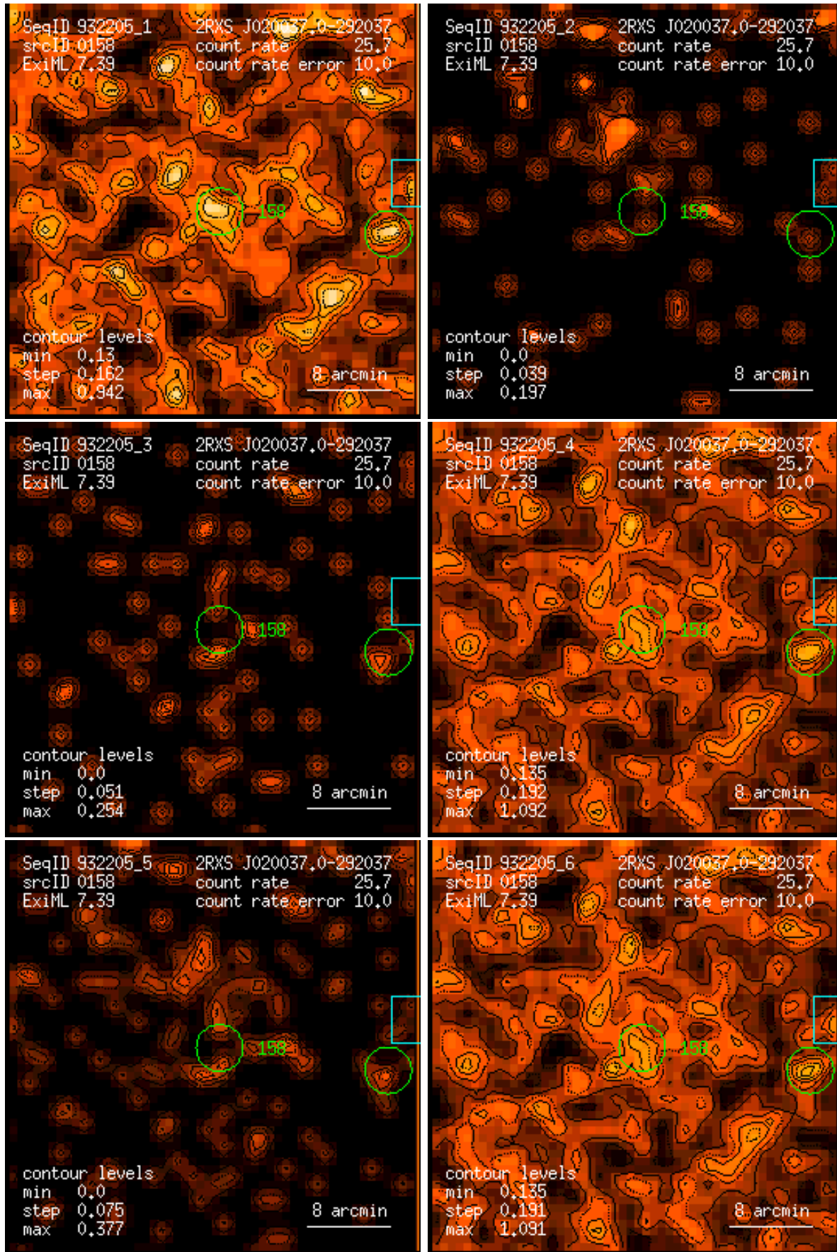
Figure 158: RASS 932205: detection 0158: band rate images, Gaussian filter: (1) PSPC channels 11 – 41, (2) 52 – 90, (3) 91 – 201, (4) 11 – 235, (5) 52 – 201, (6) 11 – 201. Broad band rates in counts/ks. Band rate contour levels in counts/ks/arcmin 2 .
