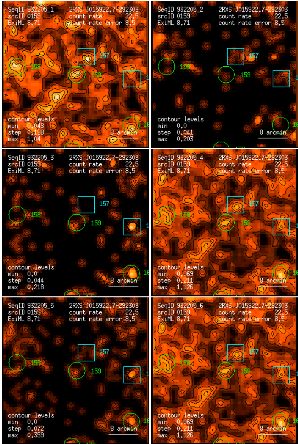
Figure 159: RASS 932205: detection 0159: band rate images, Gaussian filter: (1) PSPC channels 11 – 41, (2) 52 – 90, (3) 91 – 201, (4) 11 – 235, (5) 52 – 201, (6) 11 – 201. Broad band rates in counts/ks. Band rate contour levels in counts/ks/arcmin 2 .
