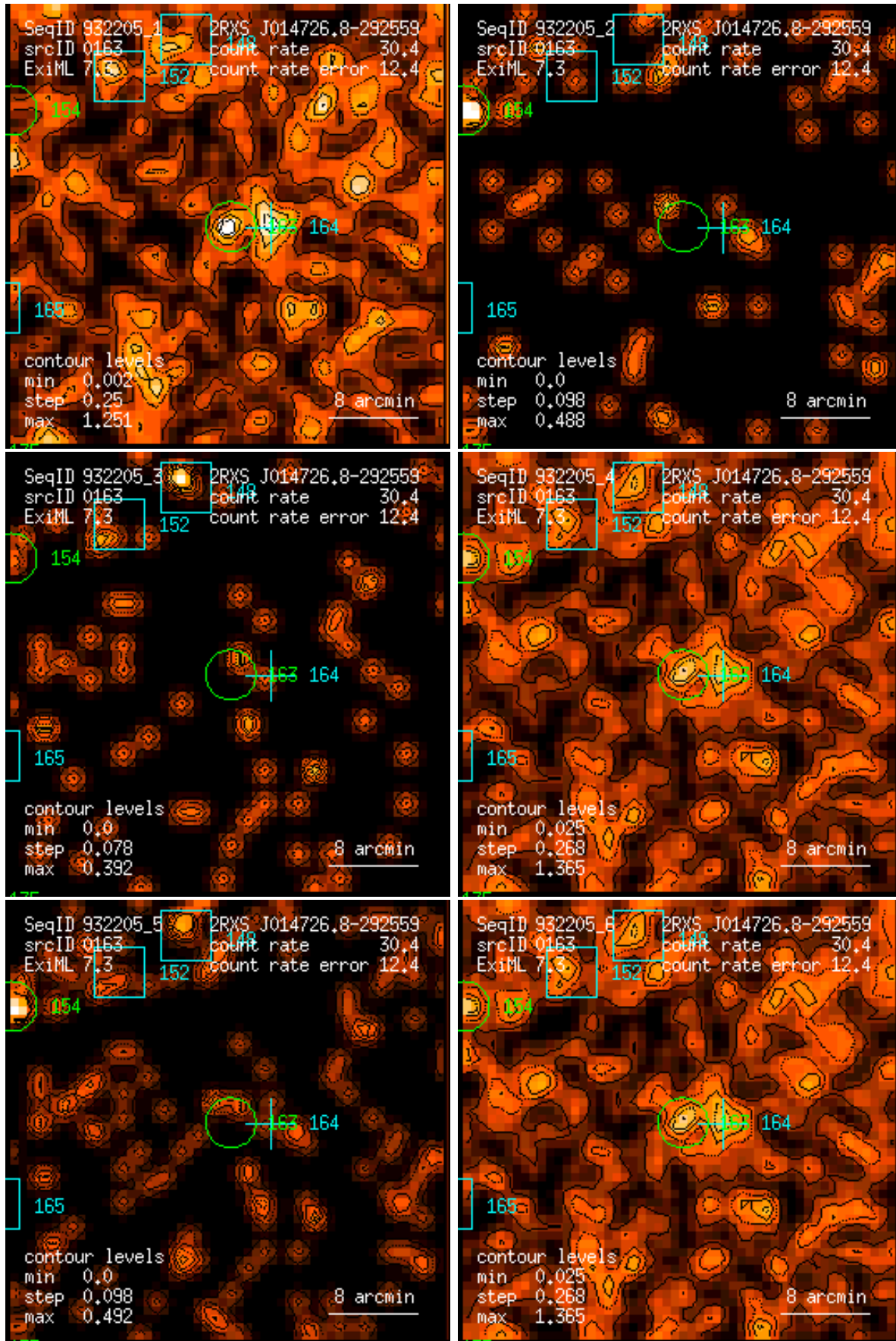
Figure 163: RASS 932205: detection 0163: band rate images, Gaussian filter: (1) PSPC channels 11 – 41, (2) 52 – 90, (3) 91 – 201, (4) 11 – 235, (5) 52 – 201, (6) 11 – 201. Broad band rates in counts/ks. Band rate contour levels in counts/ks/arcmin 2 .
