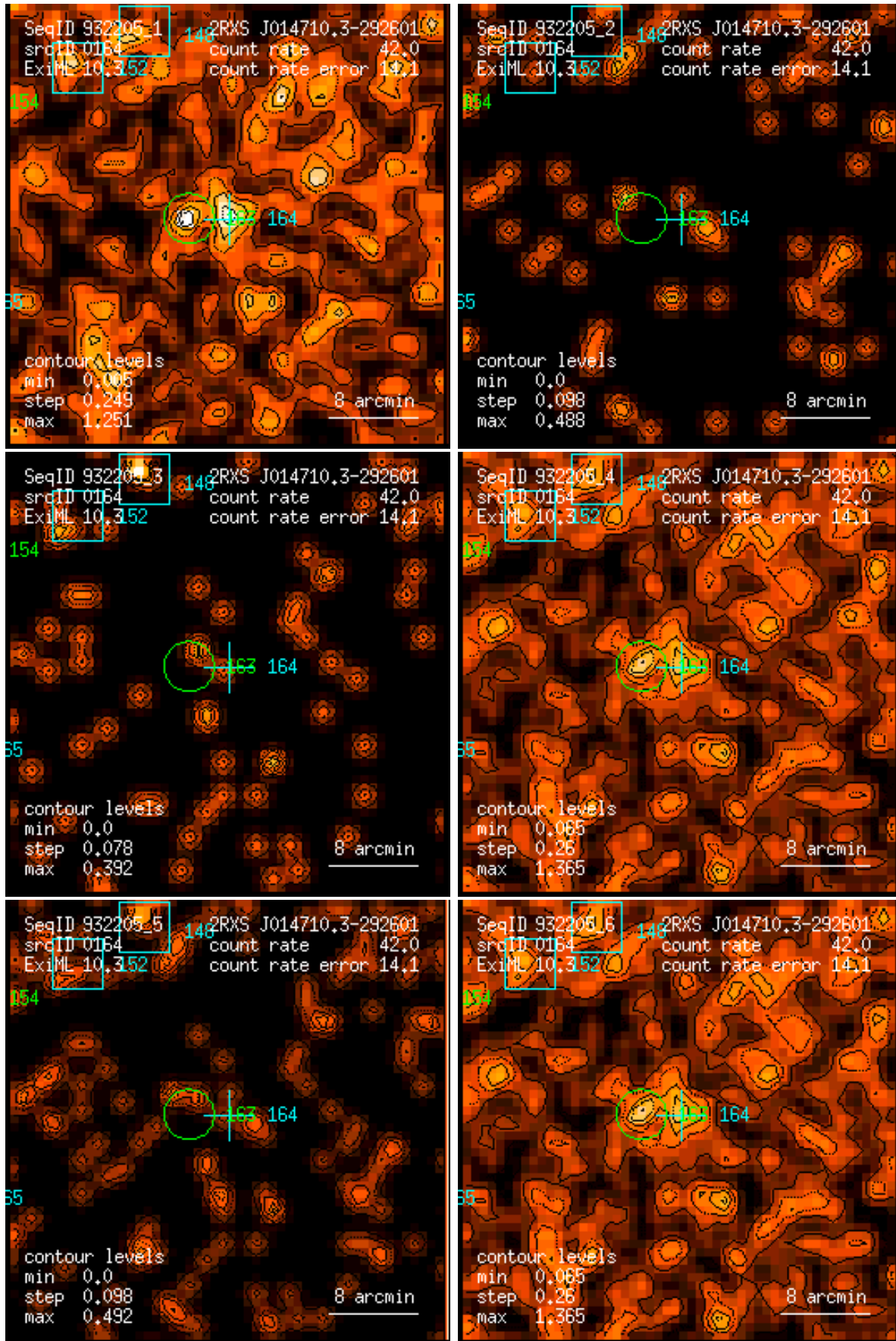
Figure 164: RASS 932205: detection 0164: band rate images, Gaussian filter: (1) PSPC channels 11 – 41, (2) 52 – 90, (3) 91 – 201, (4) 11 – 235, (5) 52 – 201, (6) 11 – 201. Broad band rates in counts/ks. Band rate contour levels in counts/ks/arcmin 2 .
