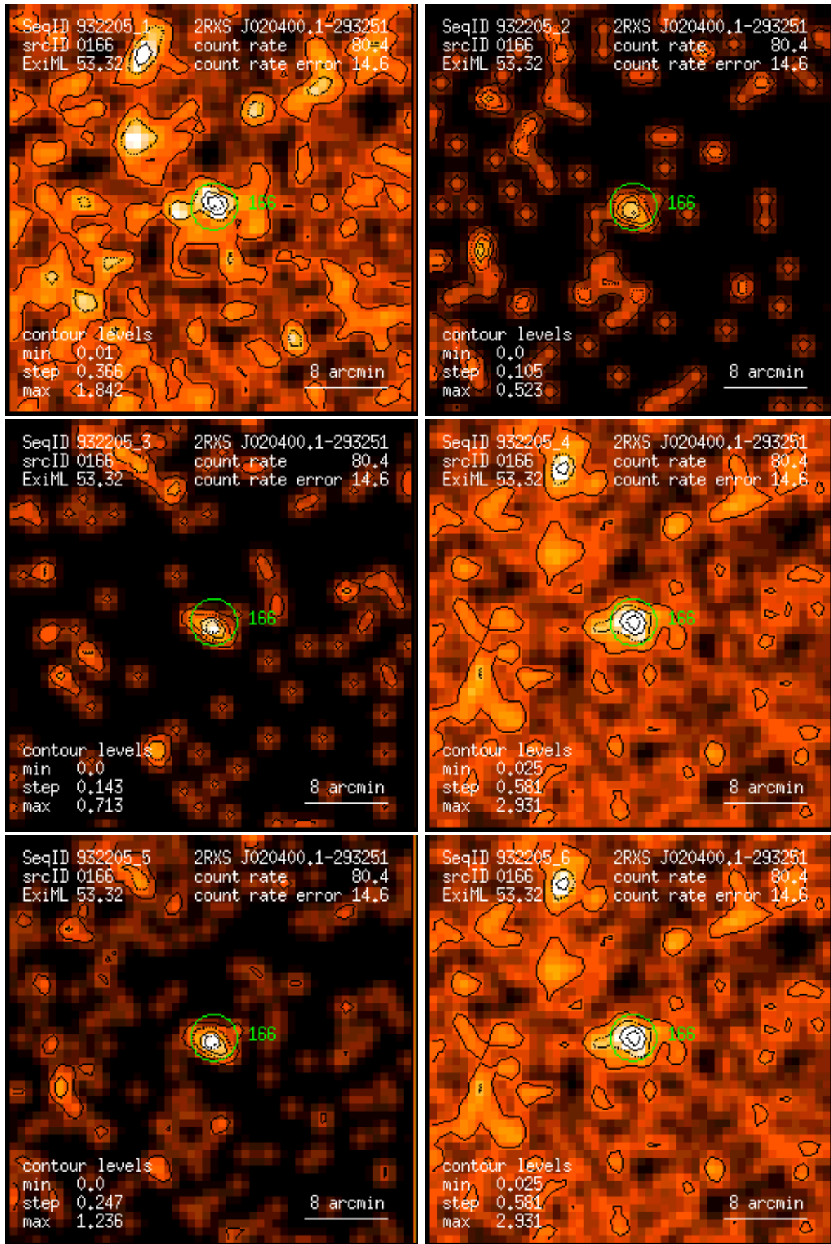
Figure 166: RASS 932205: detection 0166: band rate images, Gaussian filter: (1) PSPC channels 11 – 41, (2) 52 – 90, (3) 91 – 201, (4) 11 – 235, (5) 52 – 201, (6) 11 – 201. Broad band rates in counts/ks. Band rate contour levels in counts/ks/arcmin 2 .
