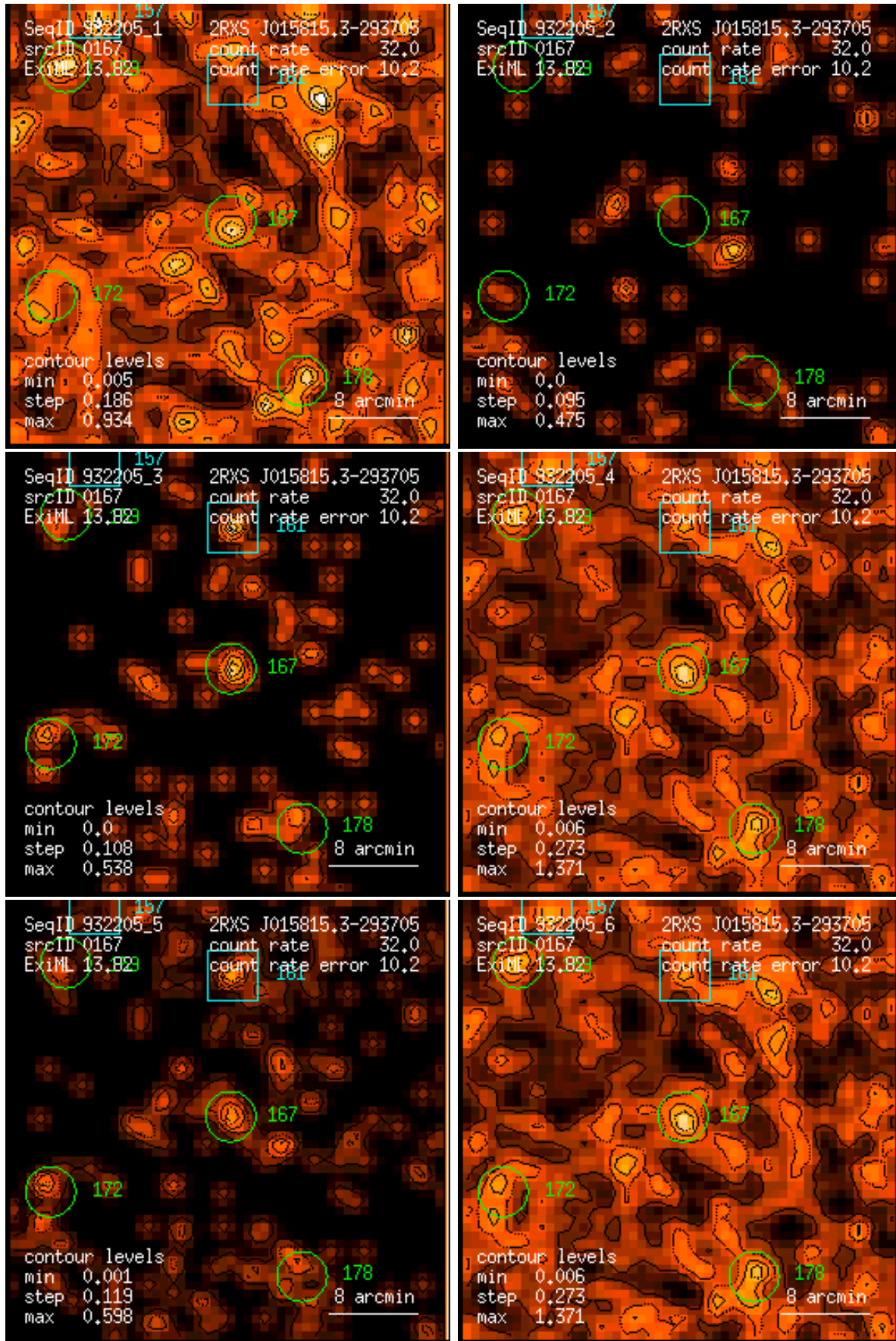
Figure 167: RASS 932205: detection 0167: band rate images, Gaussian filter: (1) PSPC channels 11 – 41, (2) 52 – 90, (3) 91 – 201, (4) 11 – 235, (5) 52 – 201, (6) 11 – 201. Broad band rates in counts/ks. Band rate contour levels in counts/ks/arcmin 2 .
