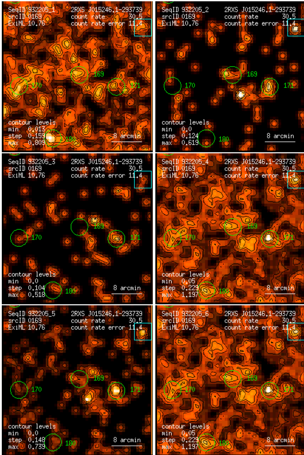
Figure 169: RASS 932205: detection 0169: band rate images, Gaussian filter: (1) PSPC channels 11 – 41, (2) 52 – 90, (3) 91 – 201, (4) 11 – 235, (5) 52 – 201, (6) 11 – 201. Broad band rates in counts/ks. Band rate contour levels in counts/ks/arcmin 2 .
