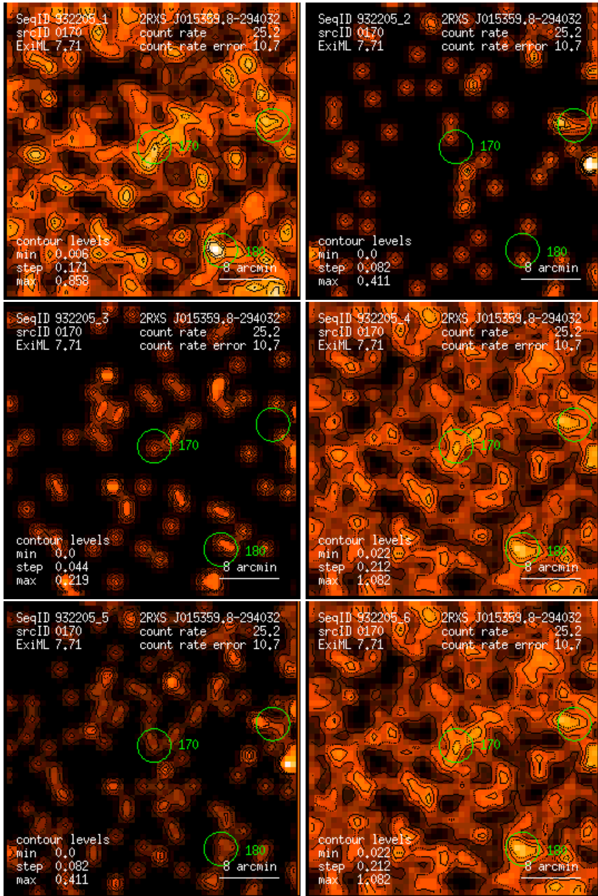
Figure 170: RASS 932205: detection 0170: band rate images, Gaussian filter: (1) PSPC channels 11 – 41, (2) 52 – 90, (3) 91 – 201, (4) 11 – 235, (5) 52 – 201, (6) 11 – 201. Broad band rates in counts/ks. Band rate contour levels in counts/ks/arcmin 2 .
