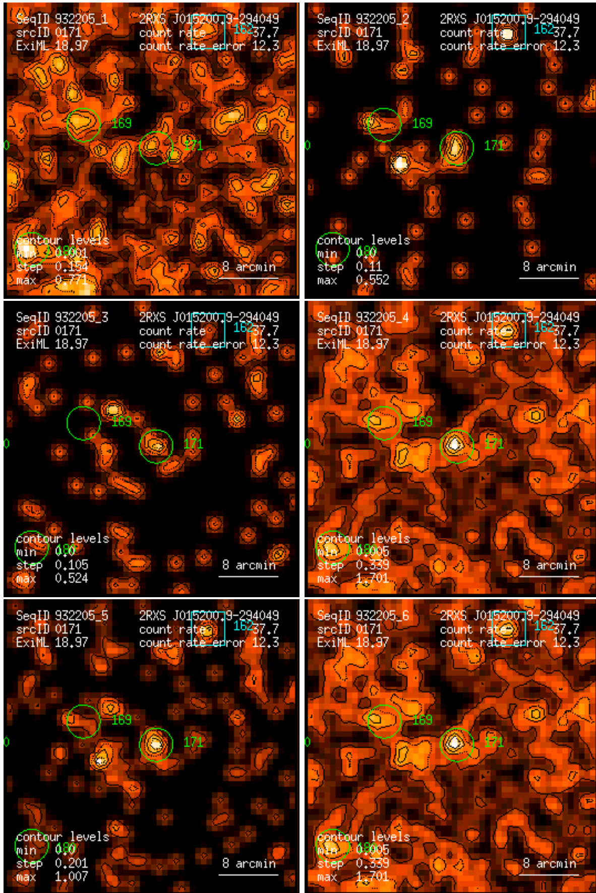
Figure 171: RASS 932205: detection 0171: band rate images, Gaussian filter: (1) PSPC channels 11 – 41, (2) 52 – 90, (3) 91 – 201, (4) 11 – 235, (5) 52 – 201, (6) 11 – 201. Broad band rates in counts/ks. Band rate contour levels in counts/ks/arcmin 2 .
