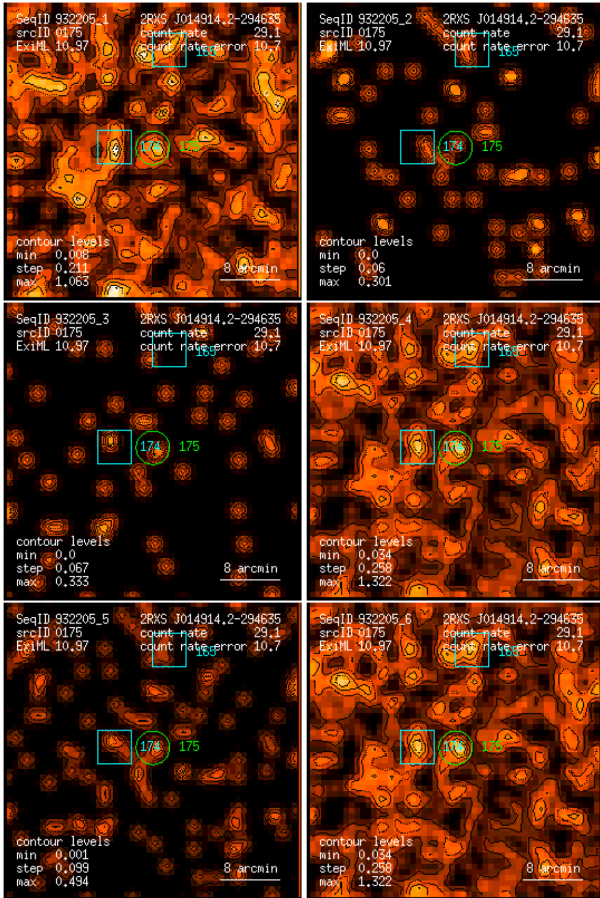
Figure 175: RASS 932205: detection 0175: band rate images, Gaussian filter: (1) PSPC channels 11 – 41, (2) 52 – 90, (3) 91 – 201, (4) 11 – 235, (5) 52 – 201, (6) 11 – 201. Broad band rates in counts/ks. Band rate contour levels in counts/ks/arcmin 2 .
