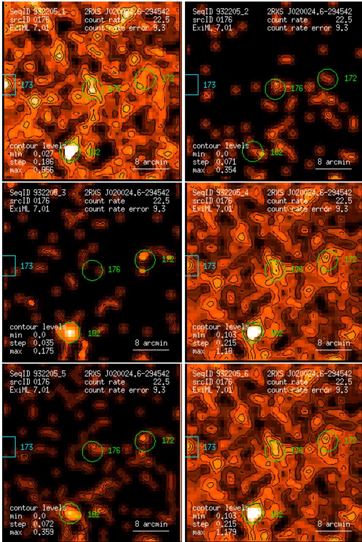
Figure 176: RASS 932205: detection 0176: band rate images, Gaussian filter: (1) PSPC channels 11 – 41, (2) 52 – 90, (3) 91 – 201, (4) 11 – 235, (5) 52 – 201, (6) 11 – 201. Broad band rates in counts/ks. Band rate contour levels in counts/ks/arcmin 2 .
