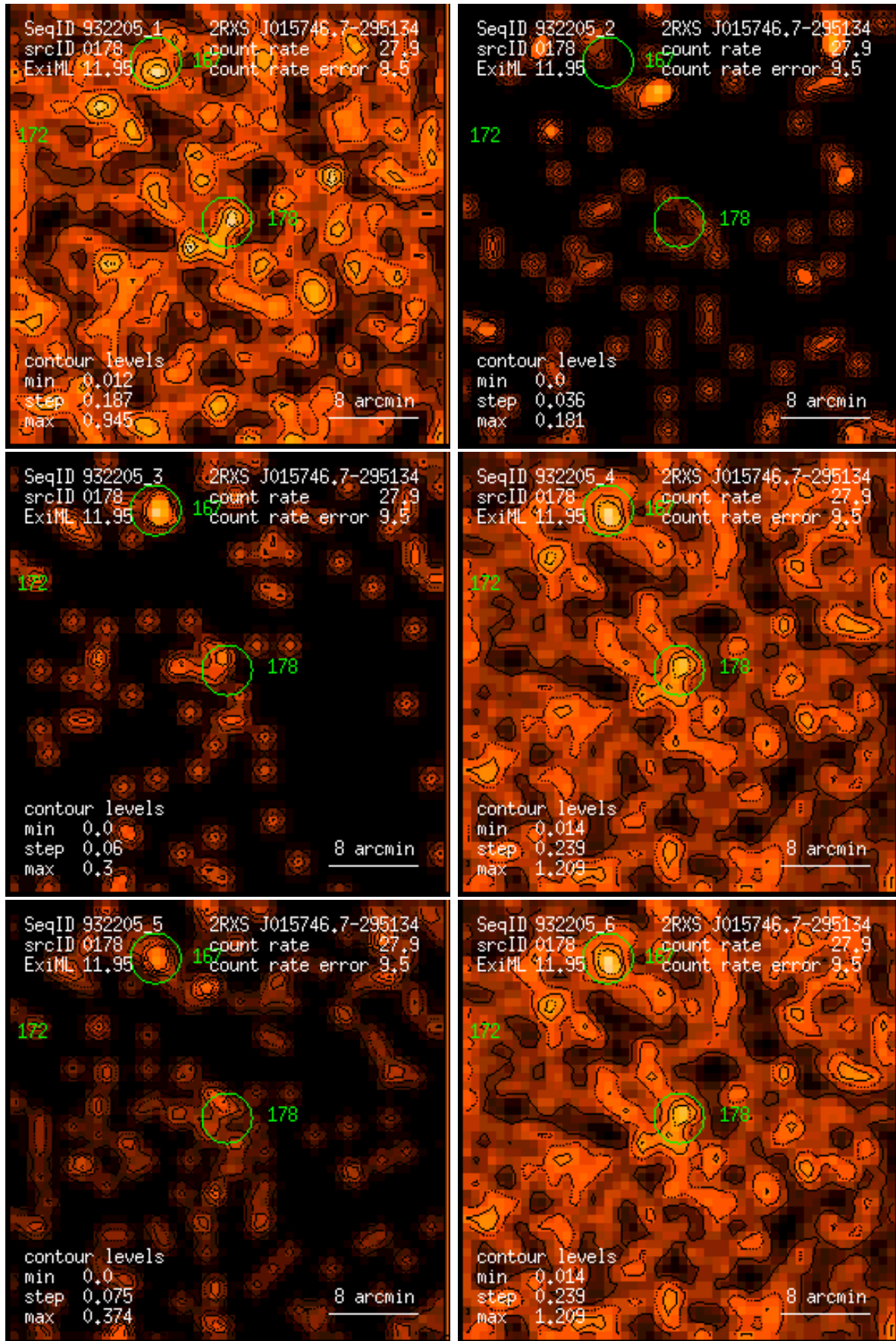
Figure 178: RASS 932205: detection 0178: band rate images, Gaussian filter: (1) PSPC channels 11 – 41, (2) 52 – 90, (3) 91 – 201, (4) 11 – 235, (5) 52 – 201, (6) 11 – 201. Broad band rates in counts/ks. Band rate contour levels in counts/ks/arcmin 2 .
