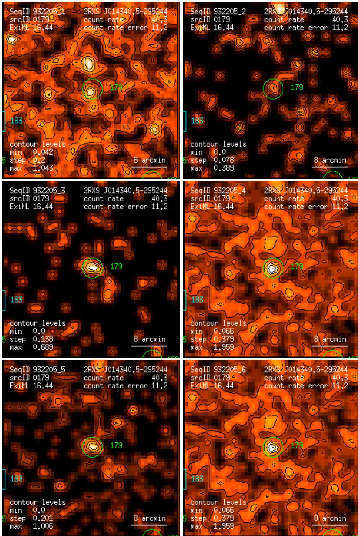
Figure 179: RASS 932205: detection 0179: band rate images, Gaussian filter: (1) PSPC channels 11 – 41, (2) 52 – 90, (3) 91 – 201, (4) 11 – 235, (5) 52 – 201, (6) 11 – 201. Broad band rates in counts/ks. Band rate contour levels in counts/ks/arcmin 2 .
