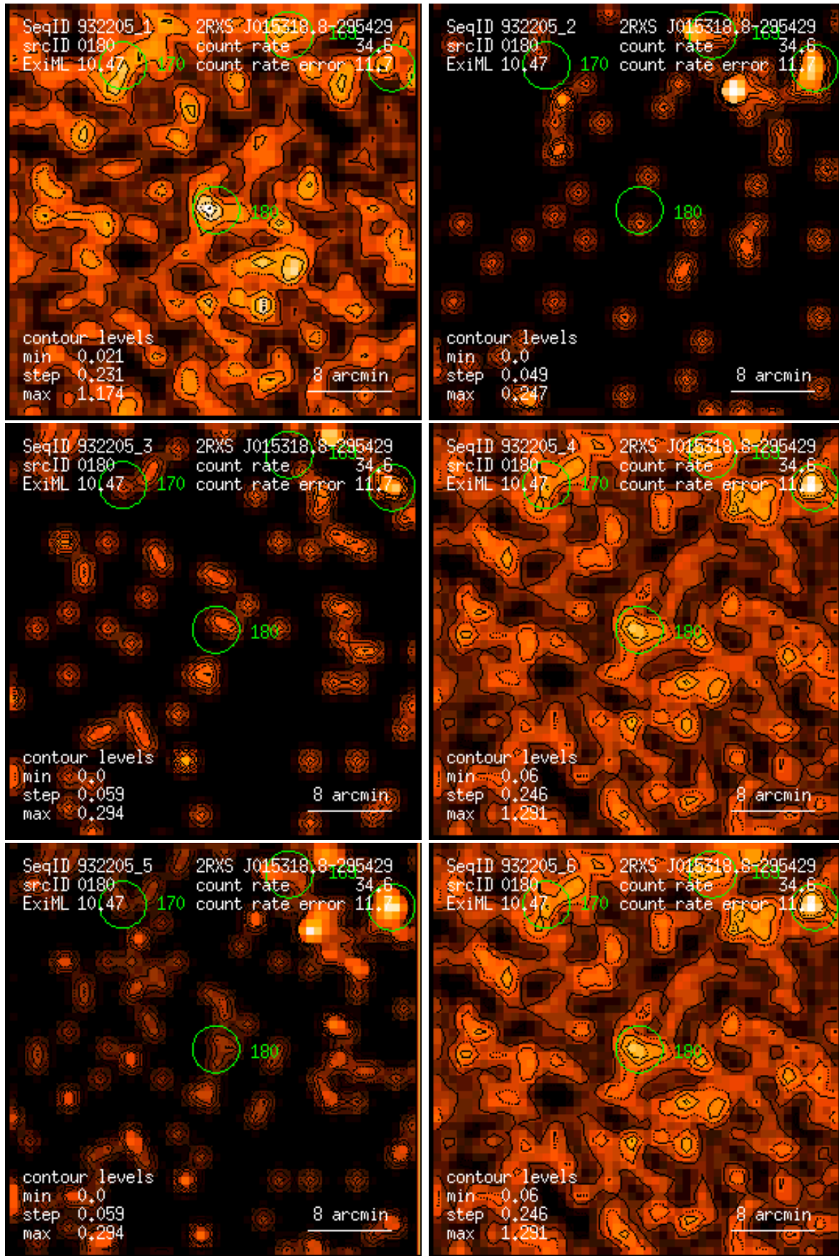
Figure 180: RASS 932205: detection 0180: band rate images, Gaussian filter: (1) PSPC channels 11 – 41, (2) 52 – 90, (3) 91 – 201, (4) 11 – 235, (5) 52 – 201, (6) 11 – 201. Broad band rates in counts/ks. Band rate contour levels in counts/ks/arcmin 2 .
