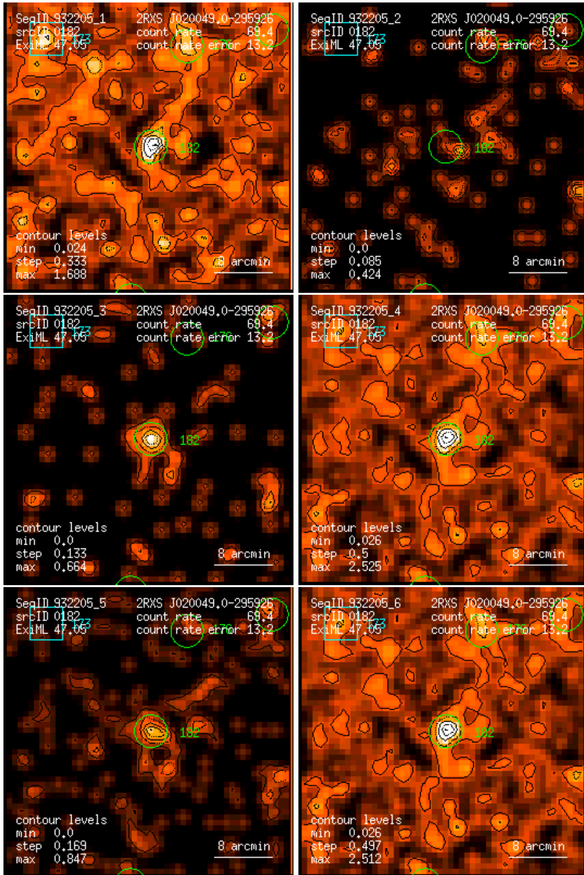
Figure 182: RASS 932205: detection 0182: band rate images, Gaussian filter: (1) PSPC channels 11 – 41, (2) 52 – 90, (3) 91 – 201, (4) 11 – 235, (5) 52 – 201, (6) 11 – 201. Broad band rates in counts/ks. Band rate contour levels in counts/ks/arcmin 2 .
