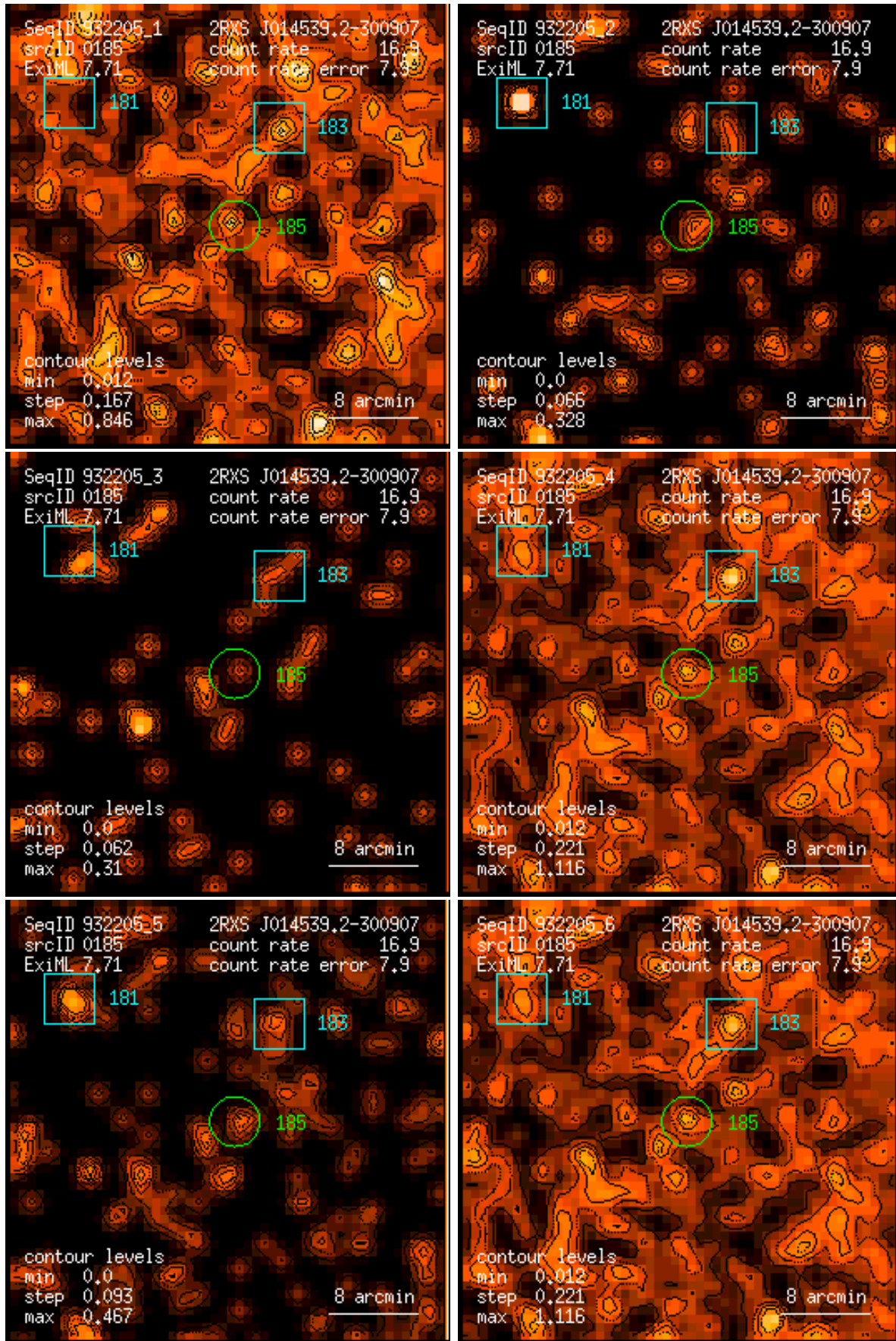
Figure 185: RASS 932205: detection 0185: band rate images, Gaussian filter: (1) PSPC channels 11 – 41, (2) 52 – 90, (3) 91 – 201, (4) 11 – 235, (5) 52 – 201, (6) 11 – 201. Broad band rates in counts/ks. Band rate contour levels in counts/ks/arcmin 2 .
