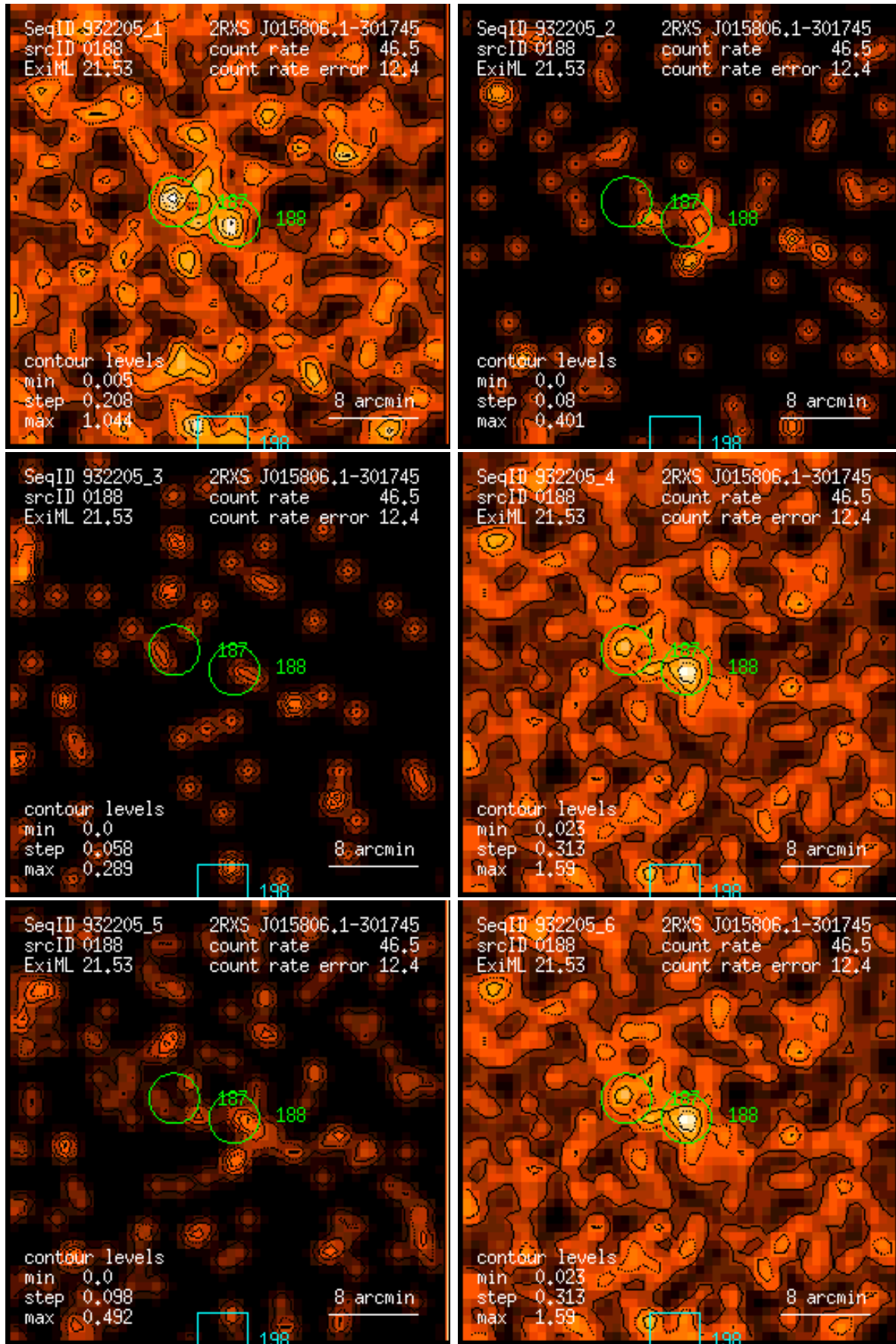
Figure 188: RASS 932205: detection 0188: band rate images, Gaussian filter: (1) PSPC channels 11 – 41, (2) 52 – 90, (3) 91 – 201, (4) 11 – 235, (5) 52 – 201, (6) 11 – 201. Broad band rates in counts/ks. Band rate contour levels in counts/ks/arcmin 2 .
