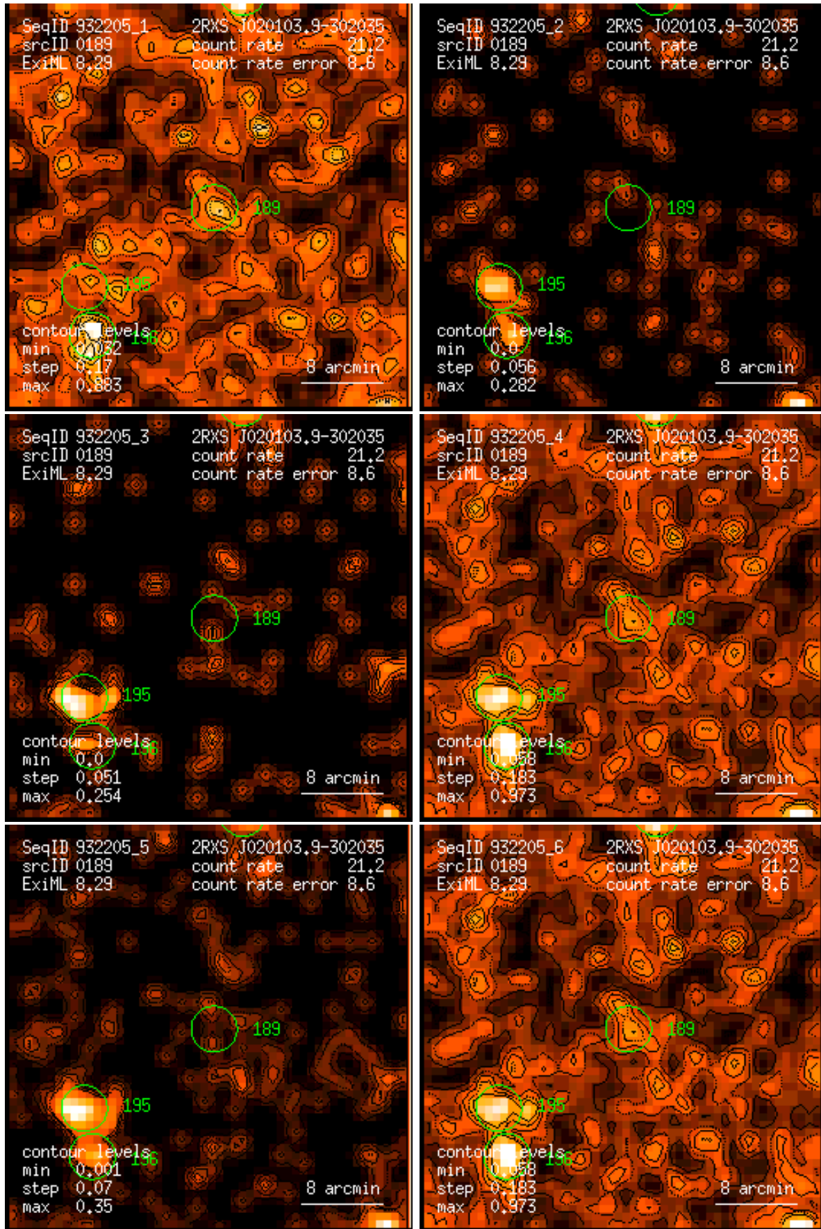
Figure 189: RASS 932205: detection 0189: band rate images, Gaussian filter: (1) PSPC channels 11 – 41, (2) 52 – 90, (3) 91 – 201, (4) 11 – 235, (5) 52 – 201, (6) 11 – 201. Broad band rates in counts/ks. Band rate contour levels in counts/ks/arcmin 2 .
