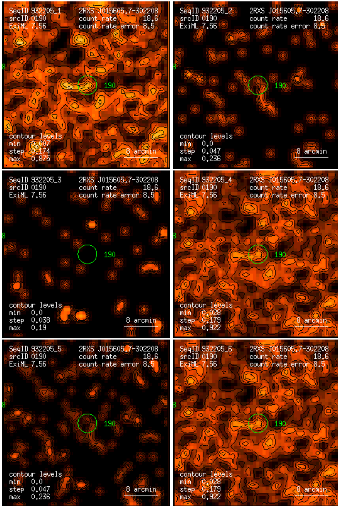
Figure 190: RASS 932205: detection 0190: band rate images, Gaussian filter: (1) PSPC channels 11 – 41, (2) 52 – 90, (3) 91 – 201, (4) 11 – 235, (5) 52 – 201, (6) 11 – 201. Broad band rates in counts/ks. Band rate contour levels in counts/ks/arcmin 2 .
